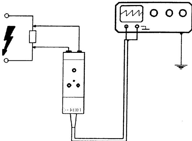
Differential probe for safe measurements
