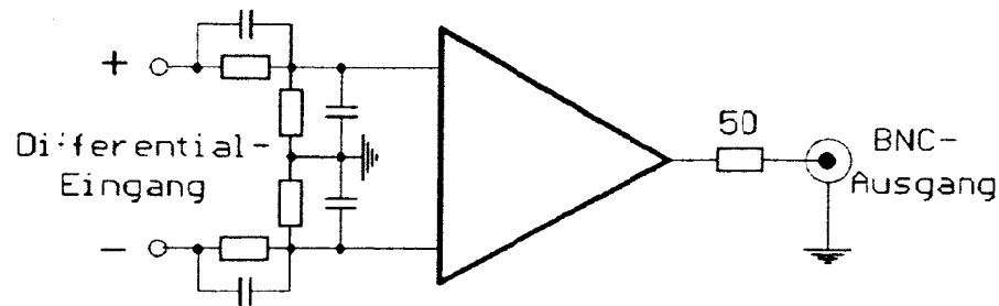
Differential probe principle
